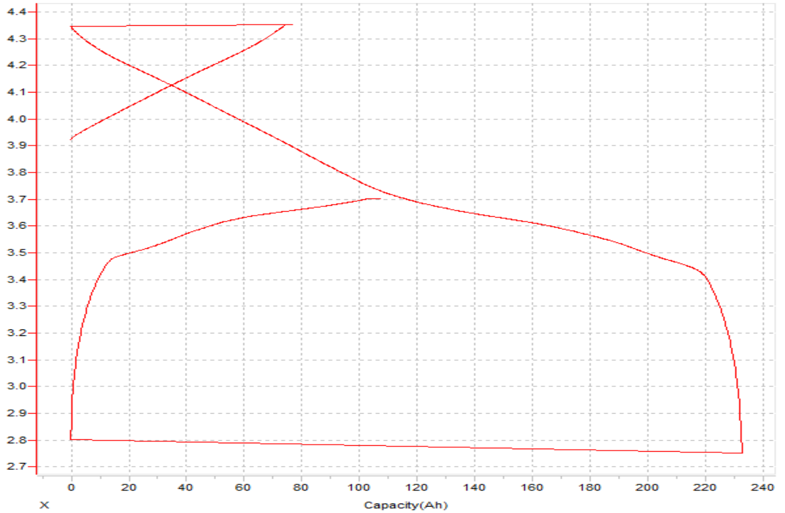
Capacity--Voltage
