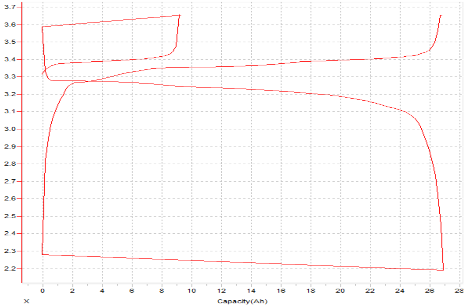
Capacity--Voltage
