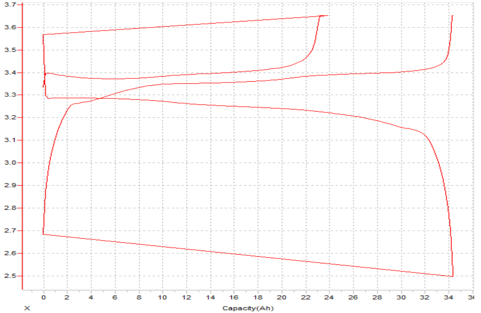
Capacity--Voltage
