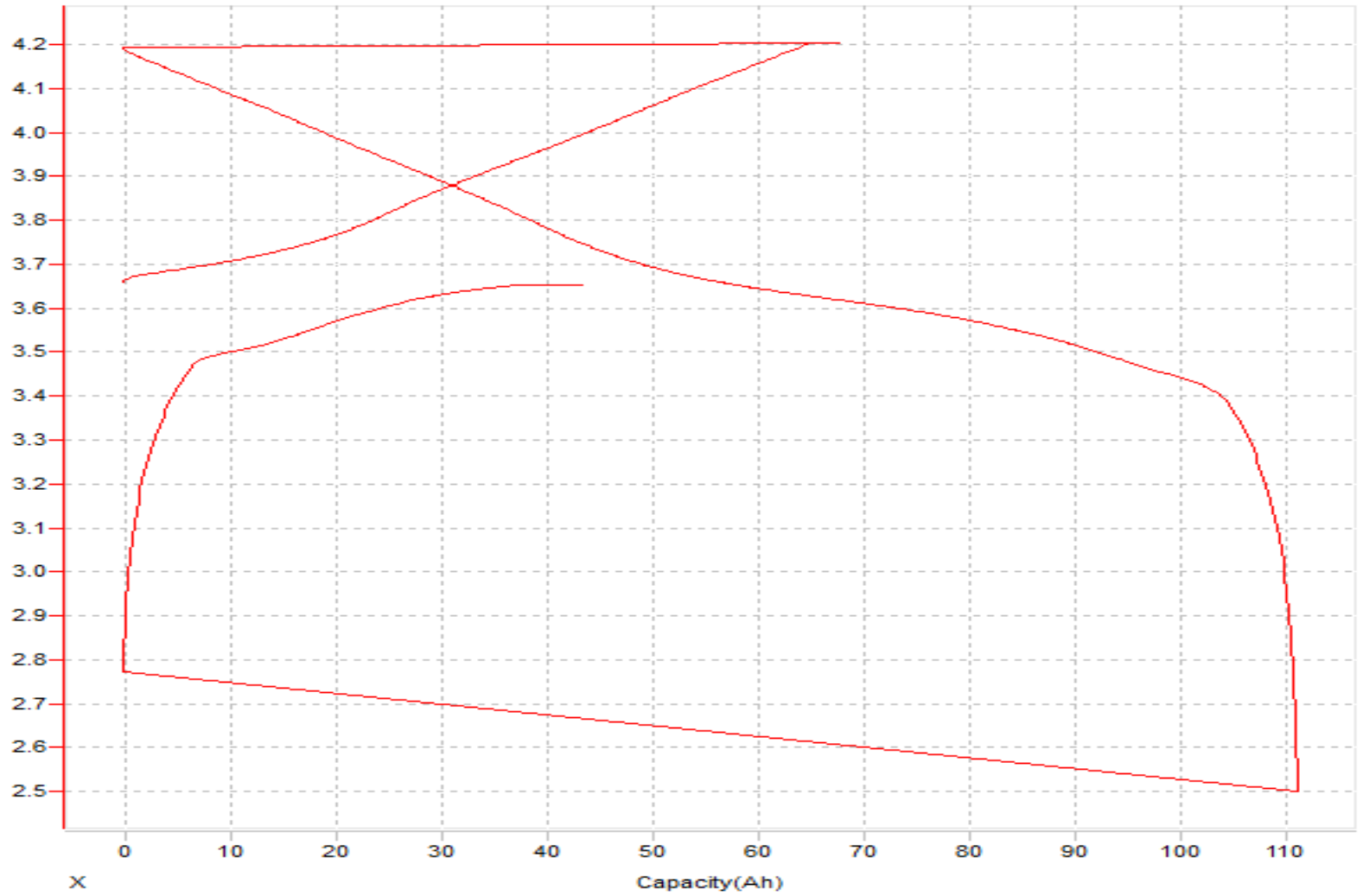
Capacity--Voltage
