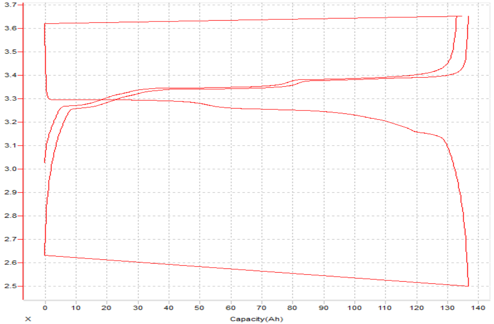
Capacity--Voltage
