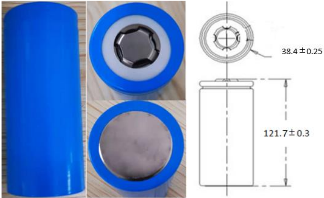
电池图片和外形尺寸 Cell appearance and dimension
